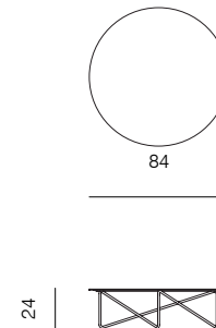
LOW TABLE Ø84 DIMENSIONS Ø84x24 CM
