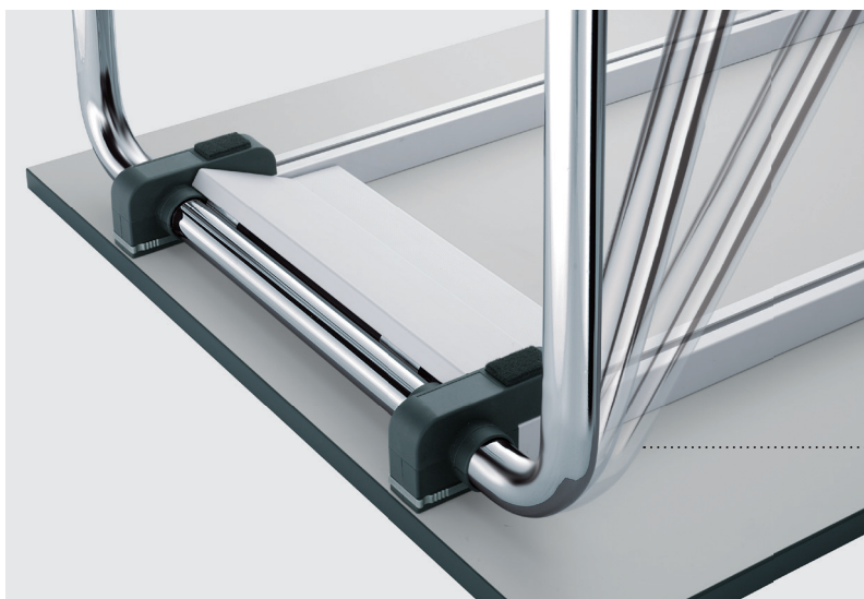
support d'empilage | mécanisme rabattant triangle de forces fermé bearing block | closing mechanism directly closing triangle of forces
